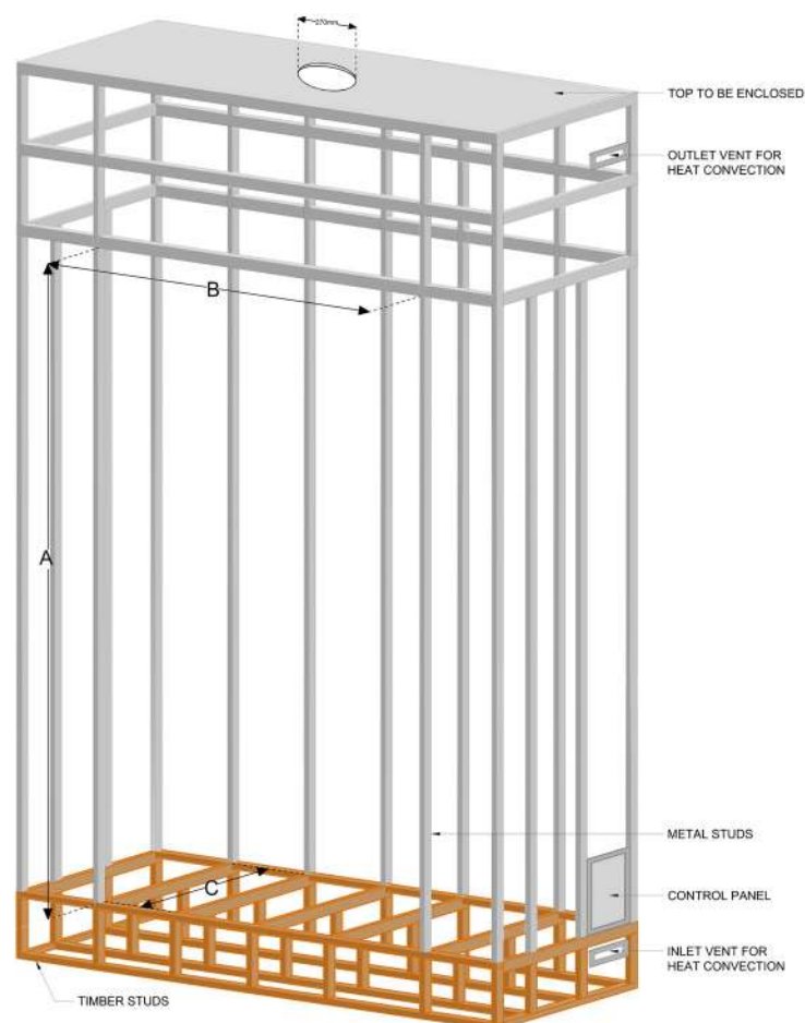
Figure 1.9 (Metal framing)
