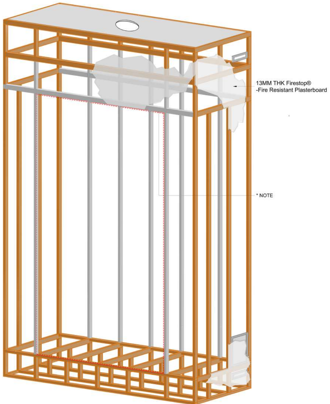
Figure 1.7 (Cladding Material)
